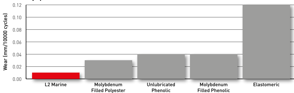
Dry Operation Wear Characteristics
